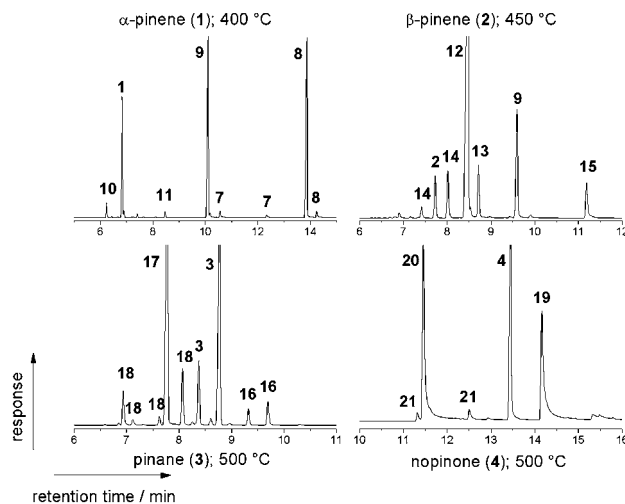
Figure 1. Gas chromatograms (GC-FID) of the liquid pyrolysis products of \alpha -pinene (1), \beta -pinene (2), pinane (3) and nopinone (4) (carrier gas: N 2 ; flow rate: 1.0 L/min; 50 \mu L starting material; solvent for dissolution of products: trichloromethane for 1, 2 and 3, ethyl acetate for 4; assigned compounds 7–21 are described in the text and a complete list of products can be found in the Supporting Information).
