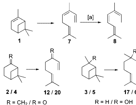
Scheme 1. Thermal decyclisation of pinane-type compounds to their acyclic isomers. [a] Ocimene ( 7 ) isomerises rapidly to the acyclic alloocimene ( 8 ) (cf. the following text).
