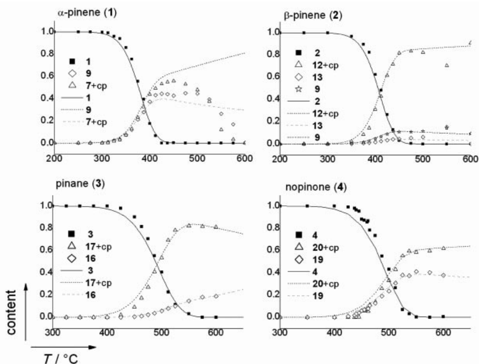
Figure 5. Simulated (lines) with experimental (symbols) data for \alpha -pinene ( 1 ), \beta -pinene ( 2 ), pinane ( 3 ) and nopinone ( 4 ) product distributions at various temperatures ( V_R : 23 mL; carrier gas: N 2 ; flow rate: 1.0 L/min; filled square: bicyclic starting material; open triangle: acyclic product and cp; open diamond/asterisk: monocyclic product).
