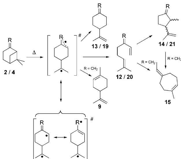
Scheme 5. Thermal isomerisation of \beta -pinene ( 2 ) and nopinone ( 4 ) (carrier gas: \text{N}_2 ; flow rate: 1.0 L/min; \beta -pinene, \text{R} = \text{CH}_2 ; nopinone, \text{R} = \text{O} ).
