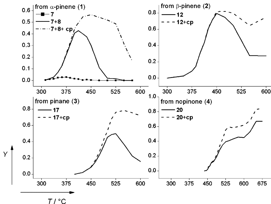
Figure 3. Yields of the acyclic and consecutive products obtained from the pyrolysis of compounds 1–4 (Figure 2) as a function of reactor temperature (carrier gas: N 2 ; flow rate: 1.0 L/min; monocyclic products are not depicted; cp = consecutive reaction products of acyclic compounds).
