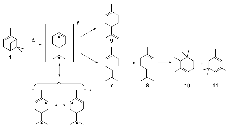
Scheme 4. Products formed by the thermal isomerisation of \alpha -pinene ( 1 ) (carrier gas: N_2 ; flow rate: 1.0 L/min).
