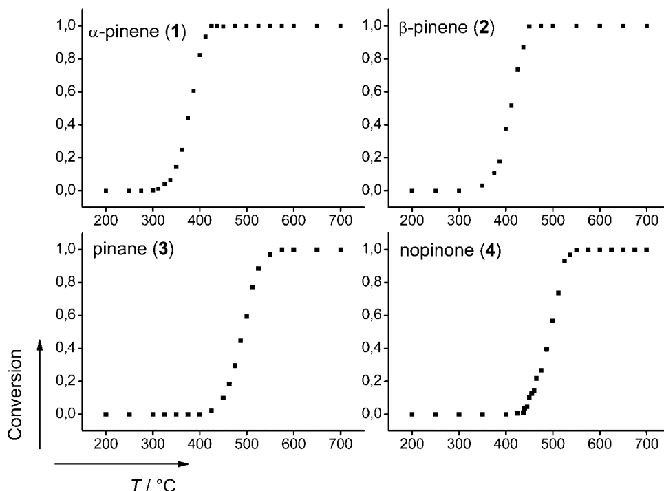
Figure 2. Conversion of compounds 1–4 in the thermal isomerisation reaction as a function of reactor temperature (carrier gas: N 2 ; flow rate: 1.0 L/min).
