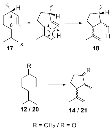
Scheme 2. Cyclisation of \beta -citronellene ( 17 ) analogues to the related cyclopentane derivatives by an ene-type reaction.
