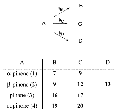
Figure 4. General reaction scheme for the kinetic investigations.
