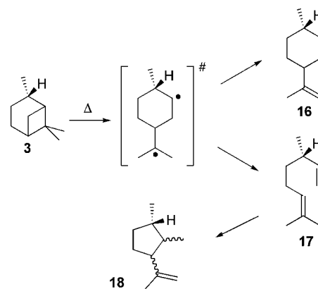
Scheme 3. Products formed by the thermal isomerisation of pinane ( 3 ) (carrier gas: N_2 ; flow rate: 1.0 L/min).
